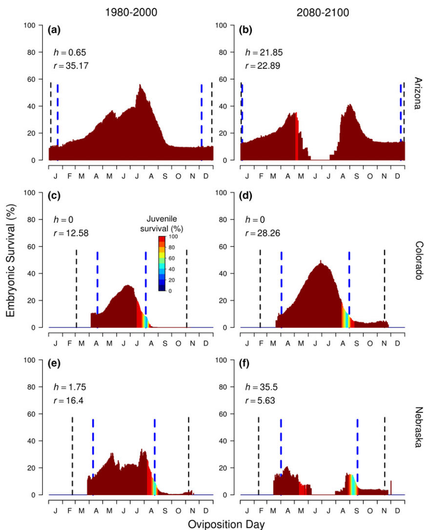
Figure 2 Predicted phenological responses to climate change in three locations: Arizona (33.87°N –111.47°E), Colorado (37.70°N –104.85°E) and Nebraska (41.13°N –101.72°E). The frequency distribution depicts the outcome of laying eggs on a certain day of year (x-axis). The height of the distribution reflects the mean percentage of embryos that survive to hatching (y-axis). The colour of the distribution denotes the mean percentage of these hatchlings that survived their first winter. The dashed black and blue lines mark the boundaries for activity and reproduction, respectively; the reproductive season was defined as the period when embryonic survival exceeds 10%. For each population, we also report the number of lethal events for embryos per year, h , and the annual rate of population growth, r .
