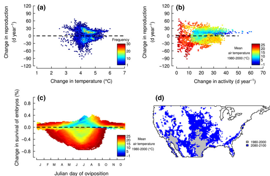
Figure 4 Impacts of climate change on opportunities for reproduction. Climate change enables lizards to reproduce earlier in spring or later in fall, but could decrease reproduction during summer (a). Symbols denote the number of locations. The effect of warming on reproduction depends on the current temperature (b); lizards in currently cool locations will have more days for successful reproduction, but lizards in currently warm locations could have many more or fewer days. The effect of warming on embryonic survivorship depends on the current temperature and the date on which eggs are laid (c). In currently warm locations, survivorship will mostly decline for potential dates of nesting. In currently cool locations, survivorship will mostly increase for eggs laid during summer. In plots a and b, symbols denote the mean of air temperatures at one or more locations. By 2080–2100, more local climates will force lizards to reproduce bimodally (d).
